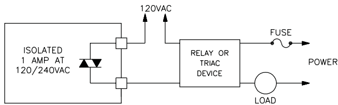
Figure 9, Triac Output
